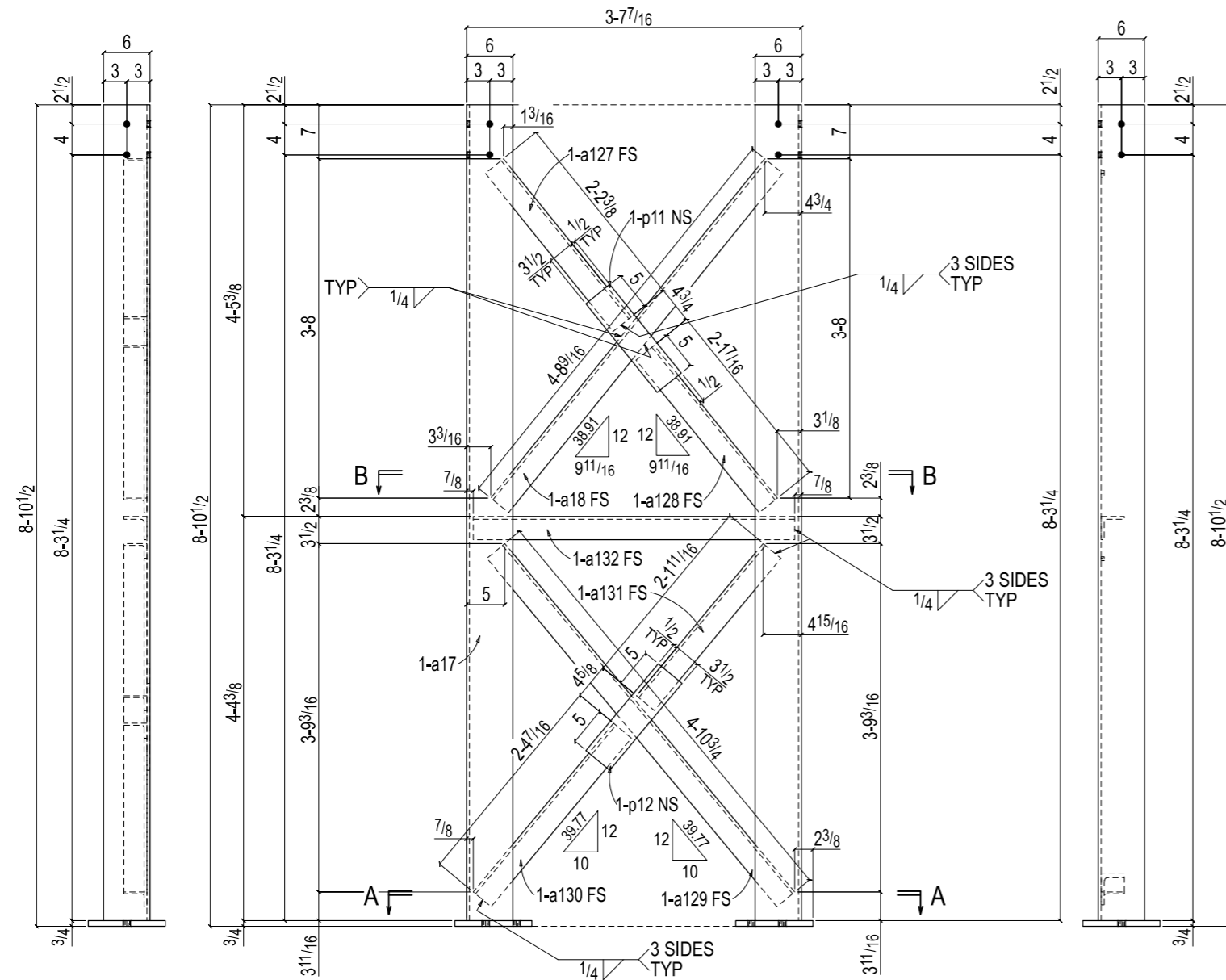
ONE FRAME 1015FR1
